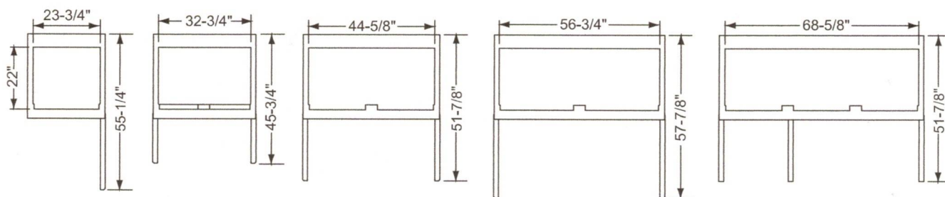
KSUR/KSUF27 PLAN VIEW
