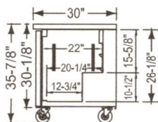
KSUR/KSUF48 ELEVATION VIEW
